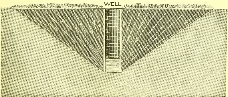
FIG. 11.—Cone of filtration.
